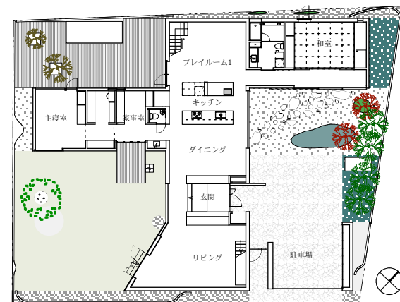
1F plan S=1/400
