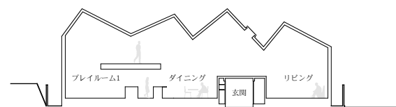
section S=1/400
